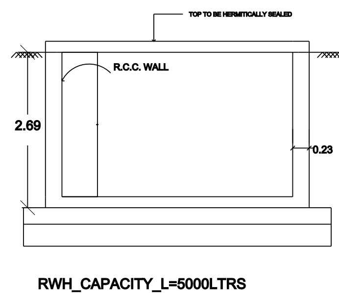
RWH_CAPACITY_L=5000LTRS
