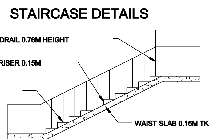
STAIRCASE DETAILS
