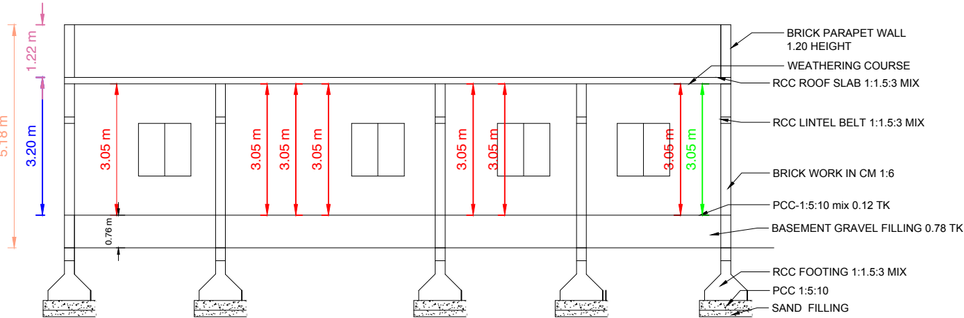
SECTION " AB "
