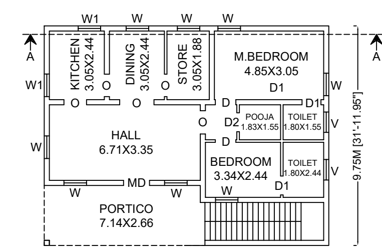
EXIST.GROUND FLOOR PLAN
