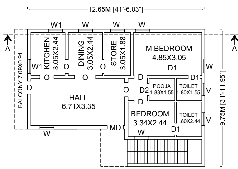
PROP.FIRST FLOOR PLAN
