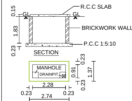
'SUMP_CAPACITY_L=6000' SUMP DETAILS
