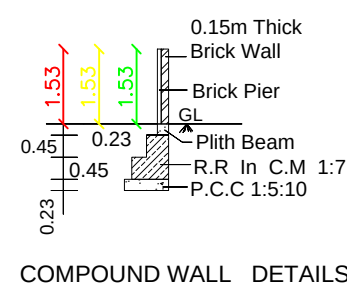
COMPOUND WALL DETAILS
