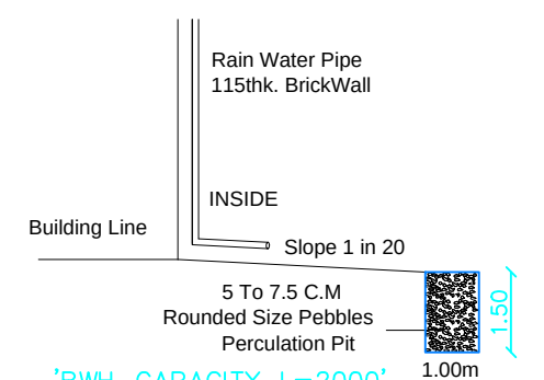
RAIN WATER HARVESTING TANK DETAILS
