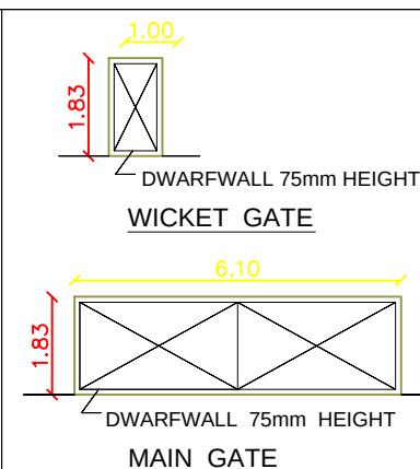
COMPOUND WALL DETAILS
