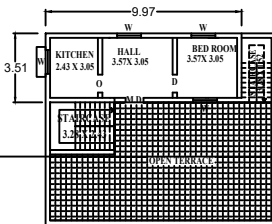
PROPOSED FIRST FLOOR
