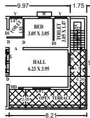
EXISTING GROUND FLOOR
