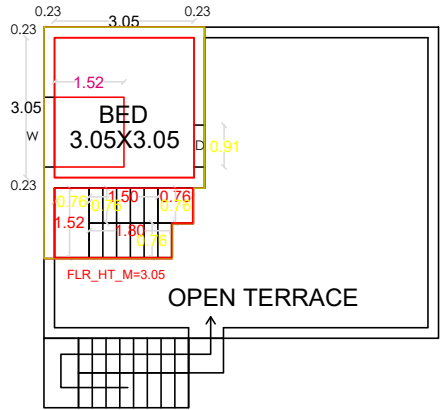
FIRST FLOOR PLAN SCALE 1 CM =1 M
