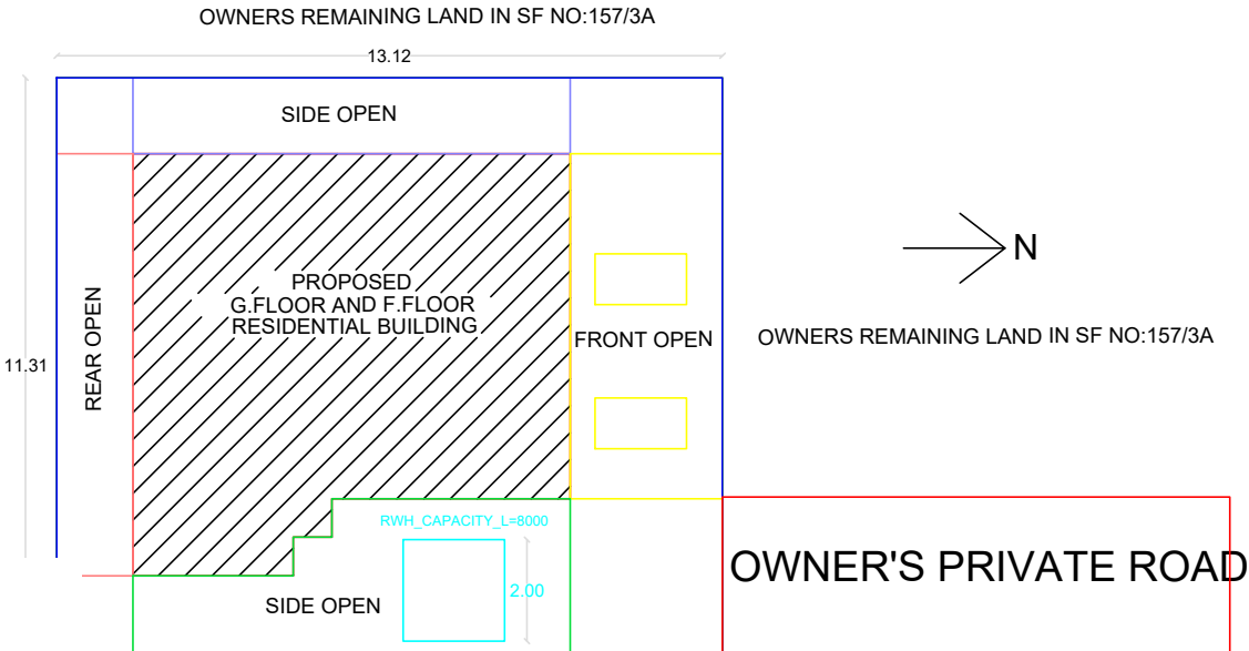
SITE PLAN SCALE 1 CM = 1 M
