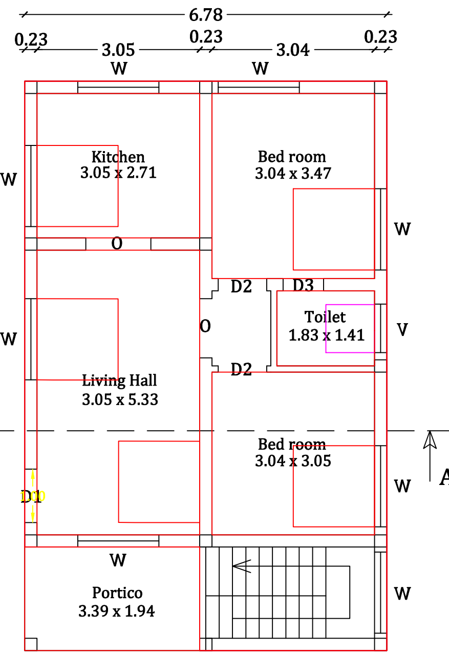
GROUND FLOOR
