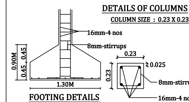
FOOTING DETAILS
