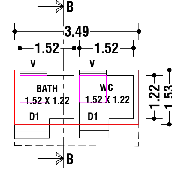
BLOCK-02 NORTH FACING GROUND FLOOR PLAN
