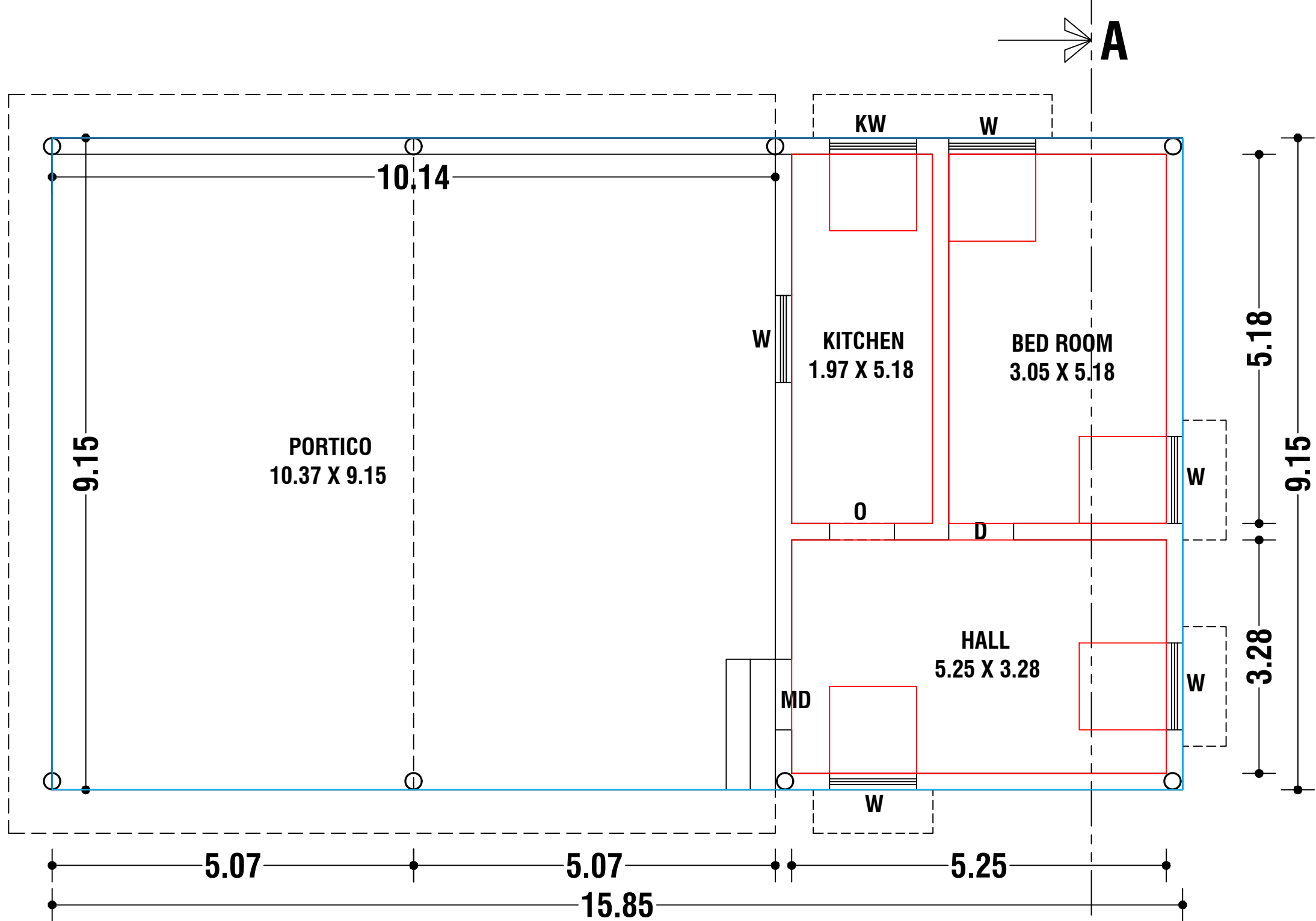
BLOCK-01 NORTH FACING GROUND FLOOR PLAN
