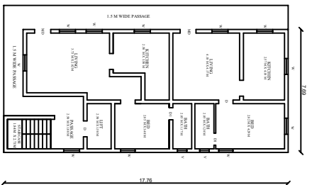
SITE PLAN SCALE 1:200
