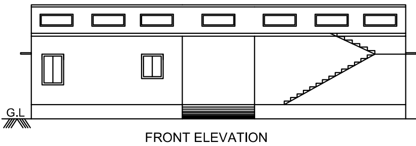
FRONT ELEVATION
