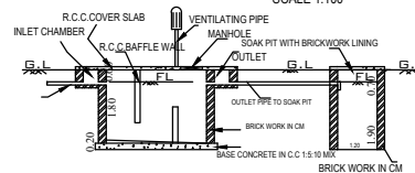
SECTIONAL DETAILS
