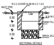
SECTIONAL DETAILS
