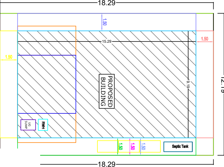
PLOT NO :- 8
