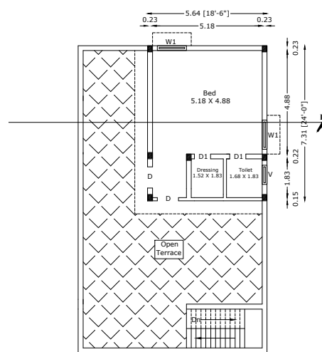
FIRST FLOOR PLAN SCALE - 1:100
