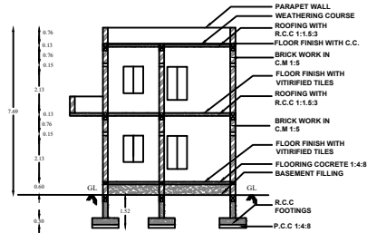
SECTION ON "S S"
