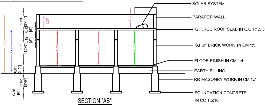
SECTION "AB"
