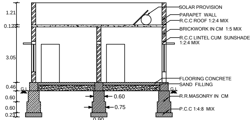
SECTION ON 'ABC'
