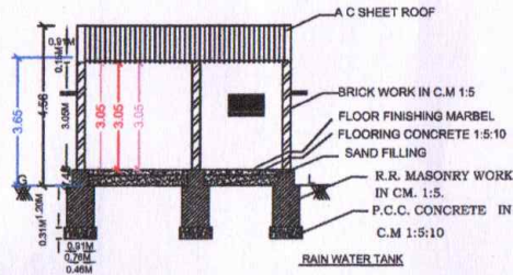
SECTION - XX
