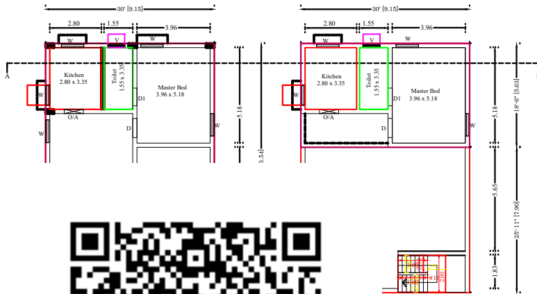
FLOOR PLAN SCALE: 1:100 (PROPOSED BUILDING)
