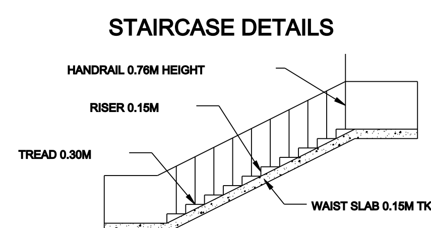
STAIRCASE DETAILS
