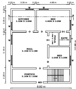
EXISTING- GROUND FLOOR - PLAN
