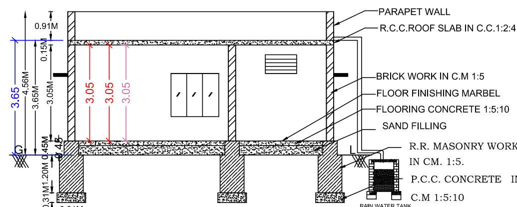
SECTION - XX
