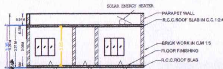
SECTION - XX
