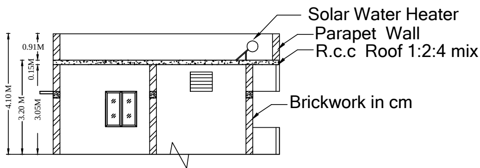
SECTION-AB
