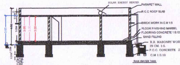
SECTION - XX
