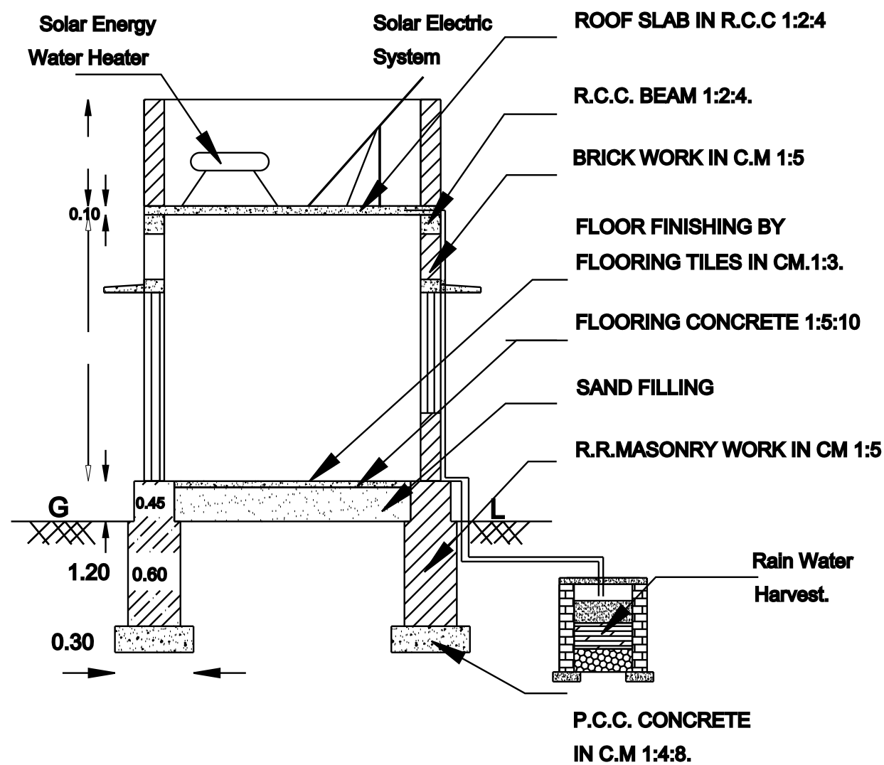
Section - XY
