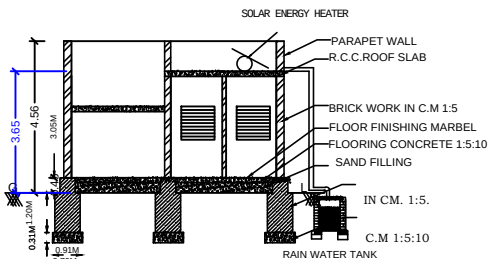
SECTION - XX
