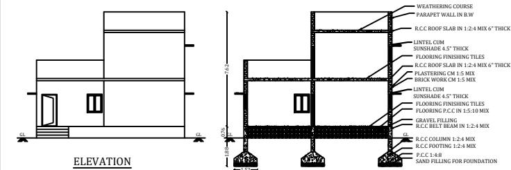
SECTION AB
