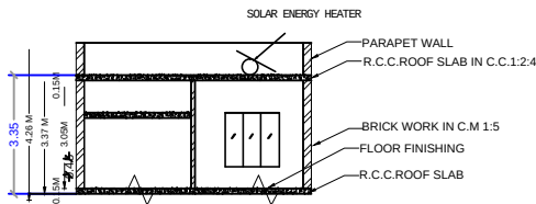
SECTION - XX
