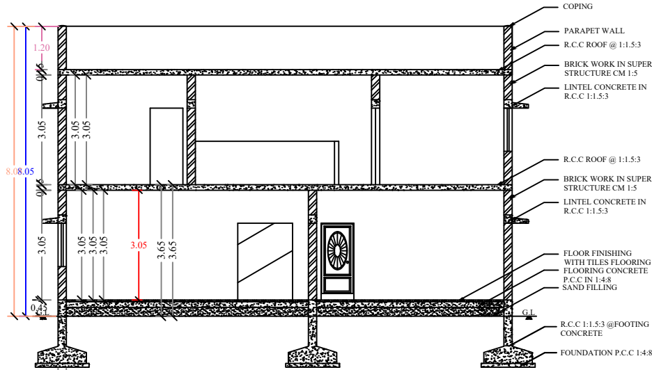
SECTION-AB
