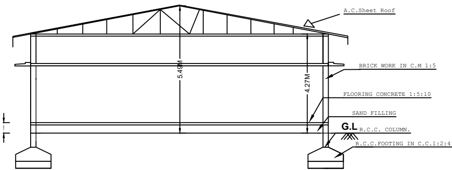
SECTION - BB1
