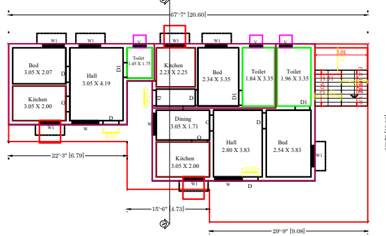
FIRST FLOOR PLAN SCALE:1:100 PROPOSED BUILDING
