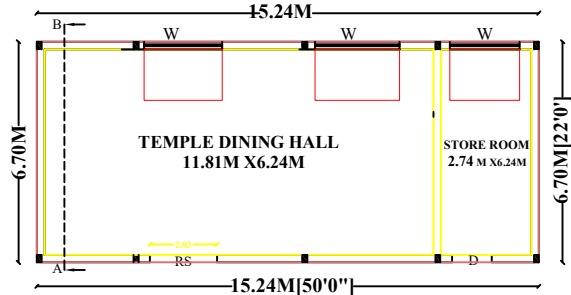
DINING & STORE ROOM - PLAN
