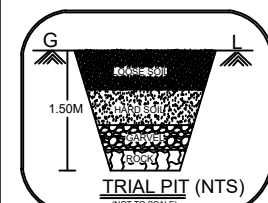
TRIAL PIT (NTS)
