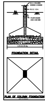
FOUNDATION DETAIL
