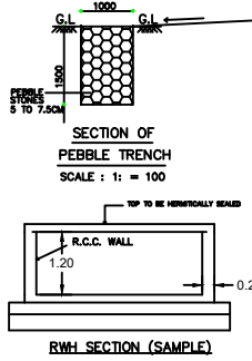
SECTION OF PEBBLE TRENCH
