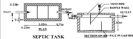
SEPTIC TANK
