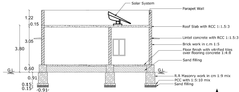
SECTION "AB"
