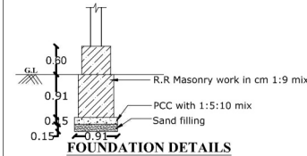
FOUNDATION DETAILS
