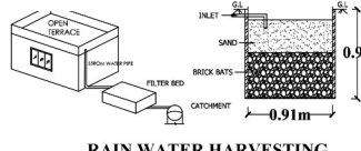
RAIN WATER HARVESTING
