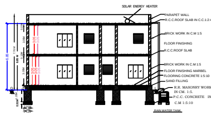
SECTION - XX
