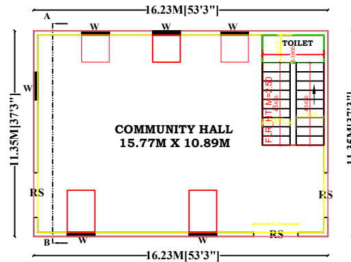
COMMUNITY HALL - PLAN
