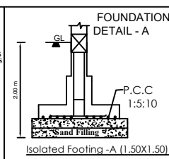
Isolated Footing -A (1.50X1.50) (Not to Scale)
