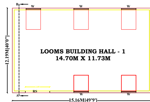
COMMERCIAL PLAN-I [LOOMS BUILDING]
