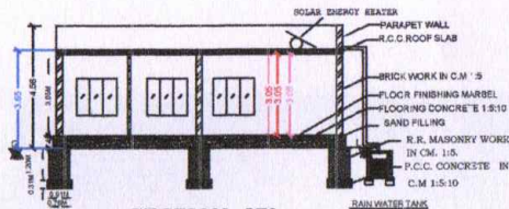
SECTION - XX
