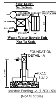
Isolated Footing - A (1.50X1.50)
