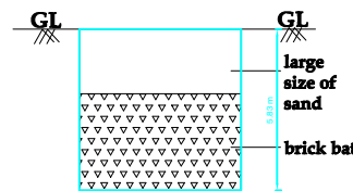
Isolated Footing - A (1.50X1.50)
