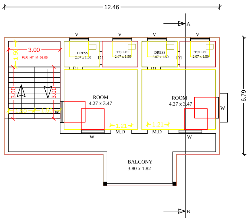
PLAN - FIRST FLOOR
