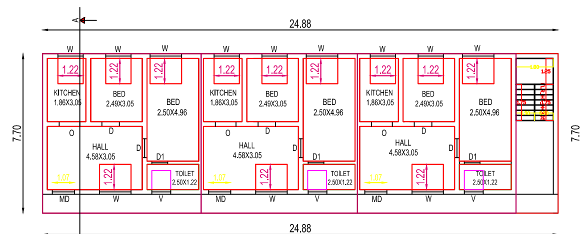
GROUND FLOOR PLAN (Scale 1:100)
