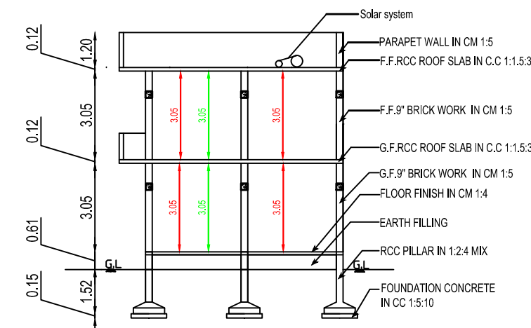
SECTION-"AA"BB"
