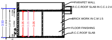
SECTION - XX
