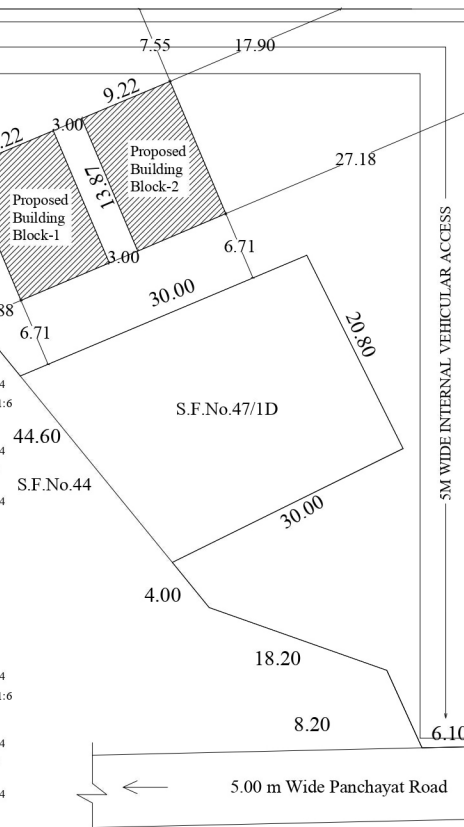
SITE PLAN
