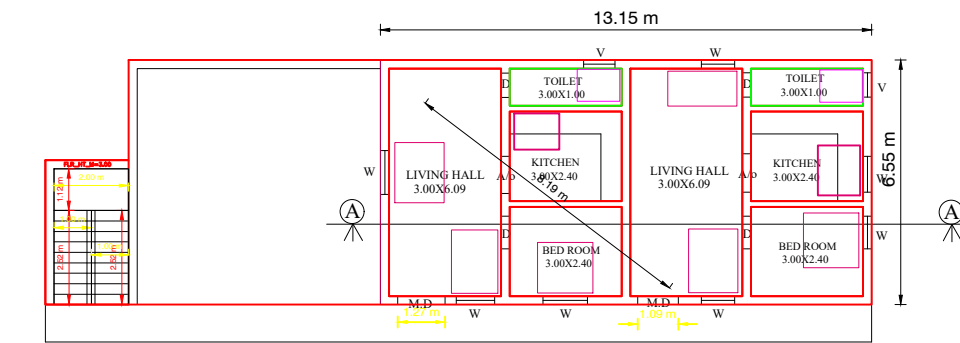
PROPOSED SECOND FLOOR
