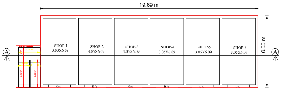
EXISTING FIRST FLOOR
