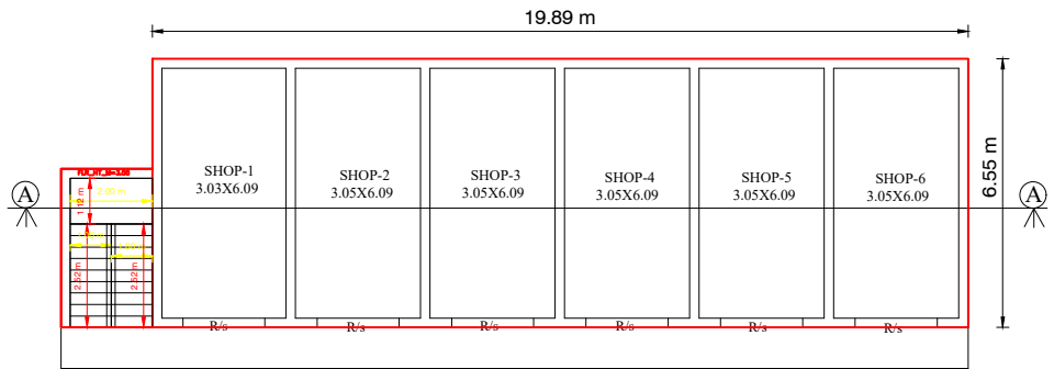
1 ST FLOOR
