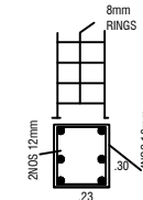
COLUMN DETAILS
