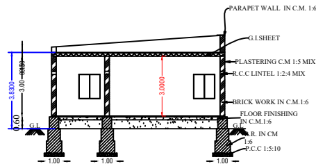
SECTION ON-"AB"
