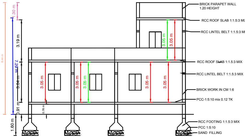
SECTION "AB"
