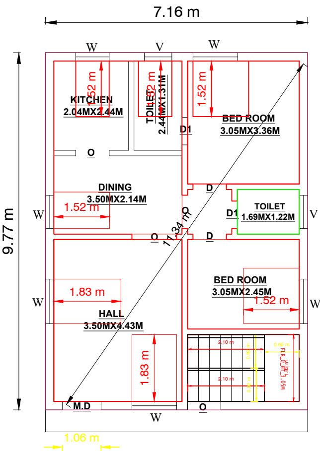
PLAN [NORTH FACING]
