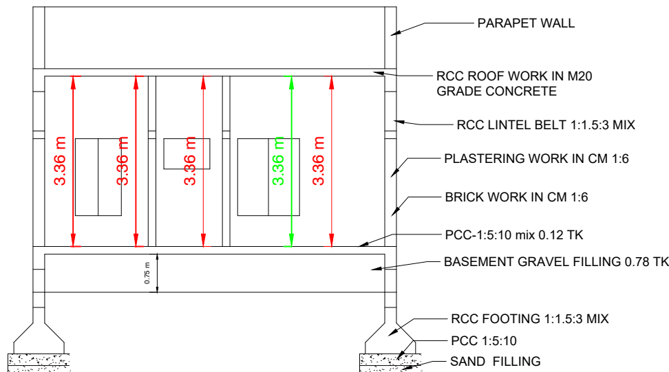
SECTION"AB"
