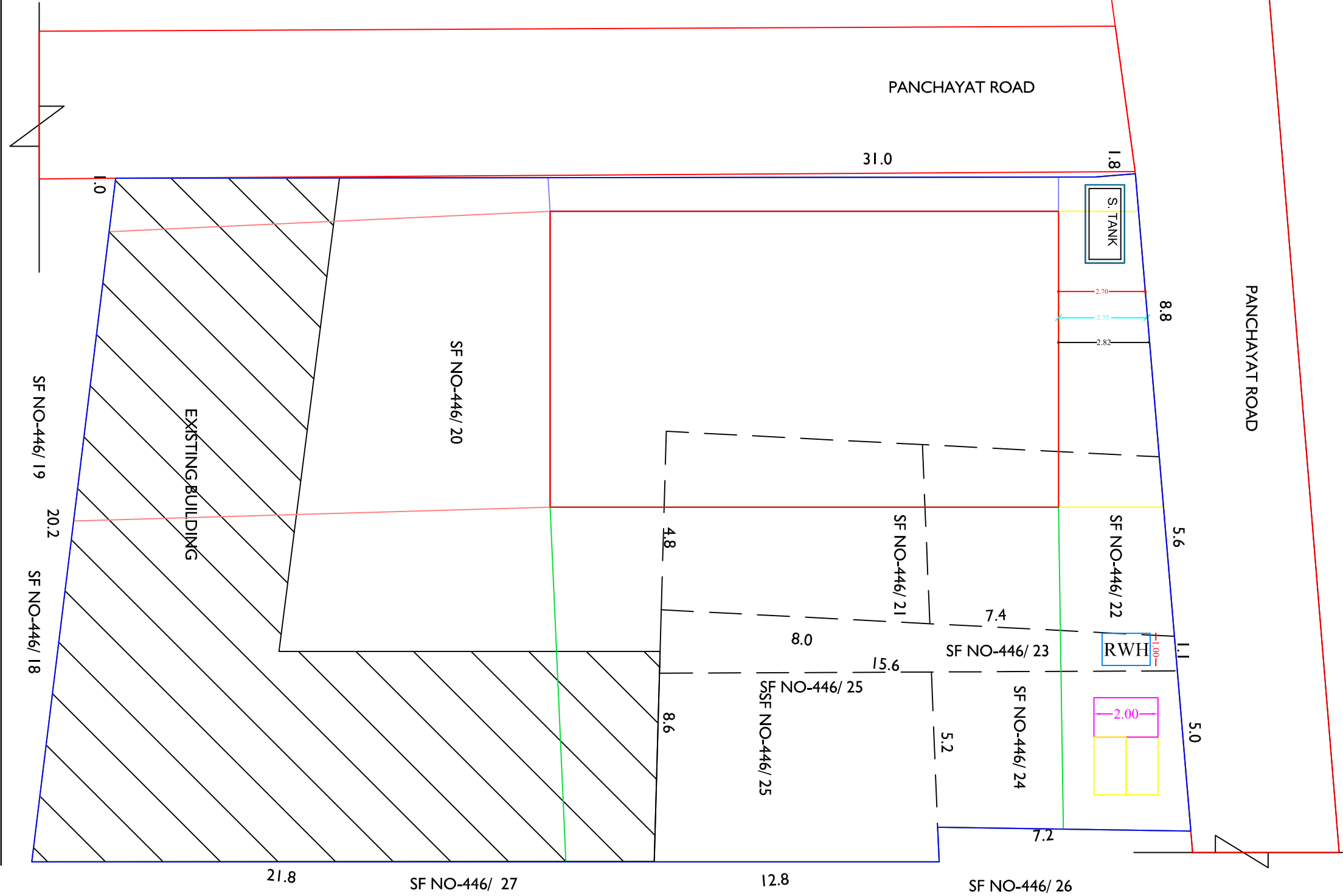
SITE PLAN
