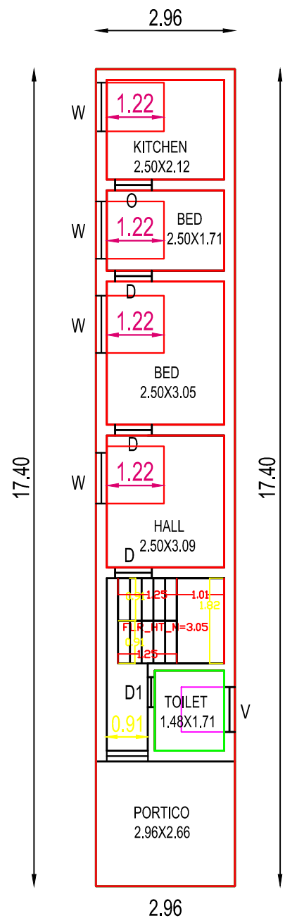
FIRST FLOOR PLAN RESIDENTIAL BUILDING
