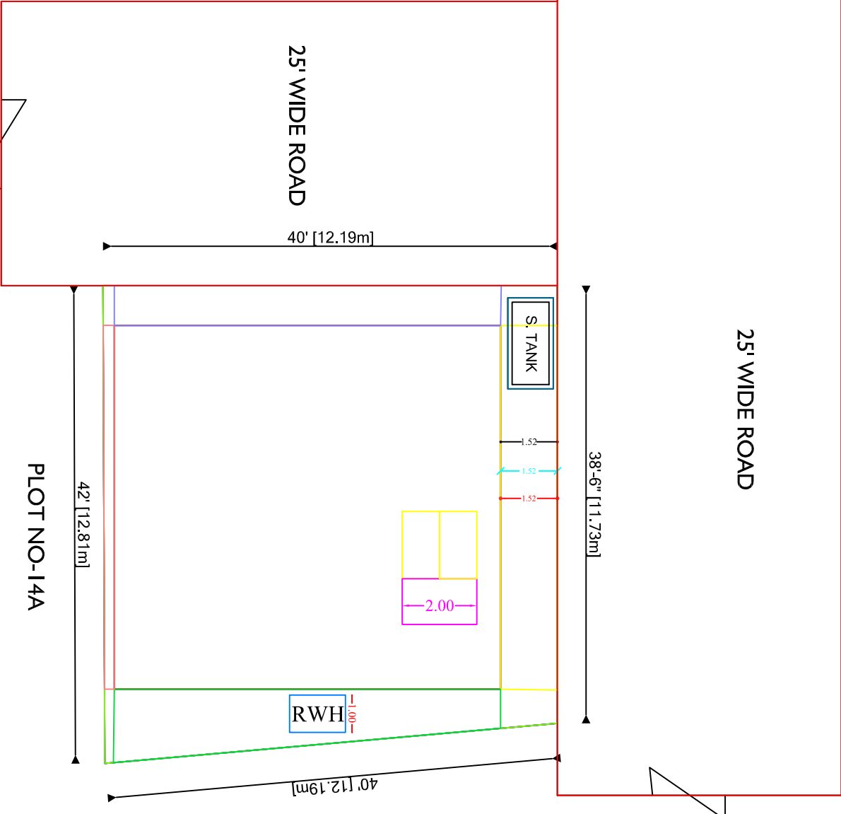
SITE PLAN
